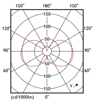
Light Distribution Diagram - MAS LEDCandleDT3.4-40W B22 927 B35CL G
